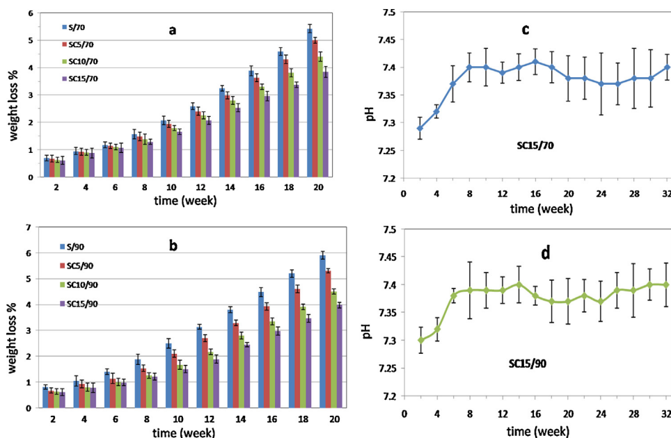
Fig. 3. (a and b) Weight loss percentage profile of the starch based scaffolds in PBS for times of 20 weeks and (c) pH changes trends of SC15/70 and (d) SC15/90 by 32 weeks.
